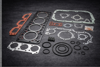
Gasket Set (Graphite) 4TNE98 (DP-546)
