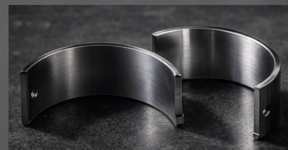
Connecting Rod Bearing (0.50) (DP)
